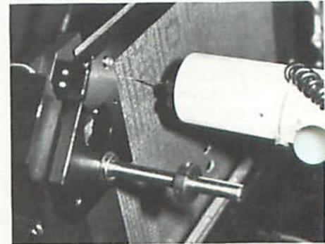
Lisa Lam, Applications engineer in robotics for the Flexible Manufacturing Technology group in Andover, at the Salem, N.H. lab where she has helped develop a robotics system for automatically probing printed circuit boards undergoing functional test. Below, a closeup of the indefector -- the part of the robot that moves the probing needle -- checking a printed circuit board located in the tester.
